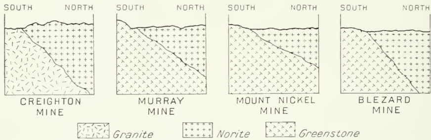
Fig. 8.—Cross-sections illustrating sill-like character of the basic edge of the norite-micropegmatite (the so-called nickel eruptive) on the southern nickel range, Sudbury, Ontario. These diagrams show that the norite-micropegmatite has partly a sill-like form.
